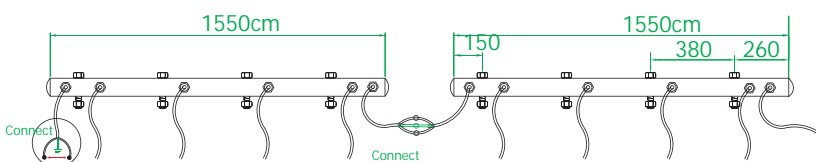
PB-604ASC wiring in 220V
